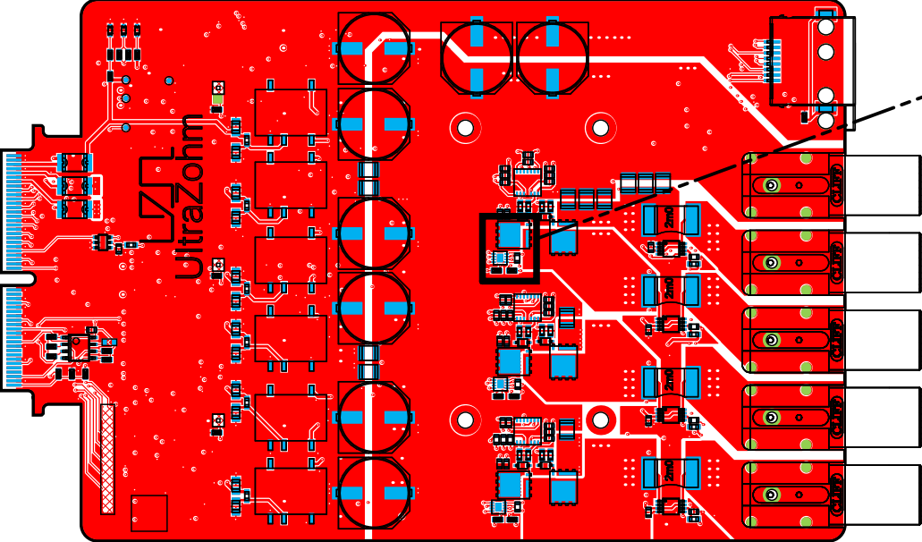
Top Component View
