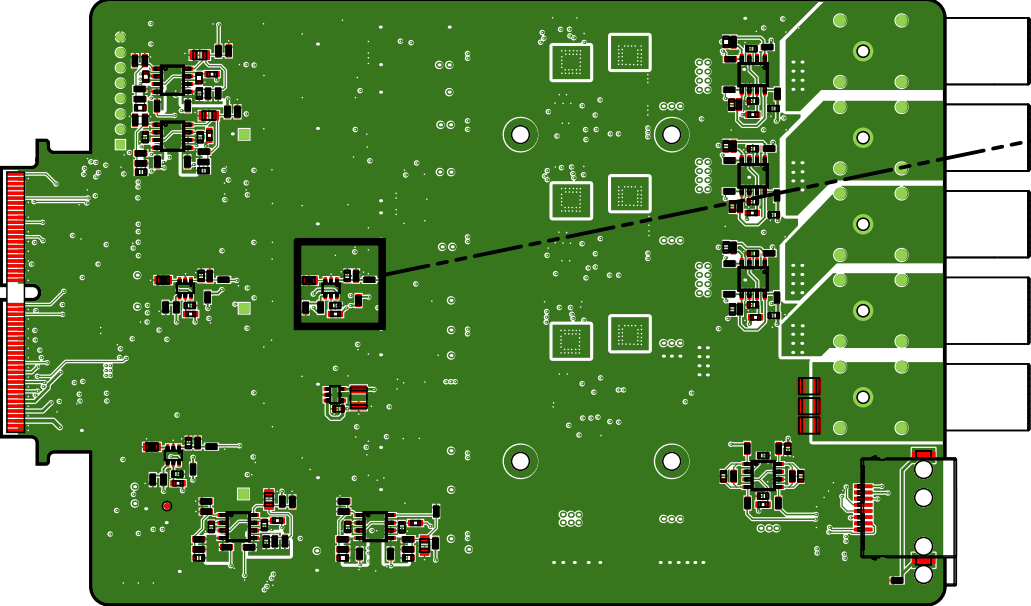
Bottom Component View
